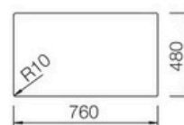
> Top Mount Cut-Out Dimensions
