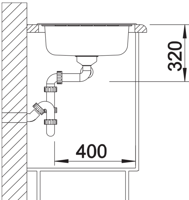
Side view
