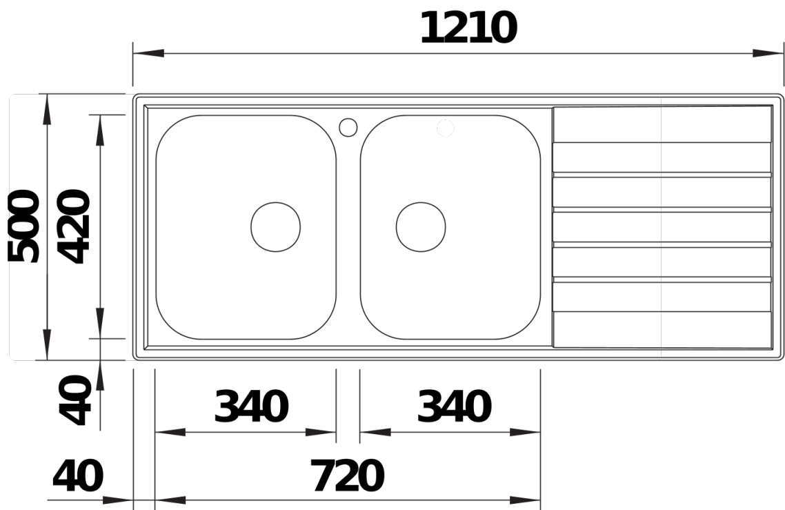
Top view
