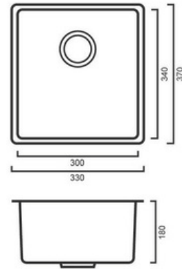
TECH60U: 330mm x 370mm x 180mm
